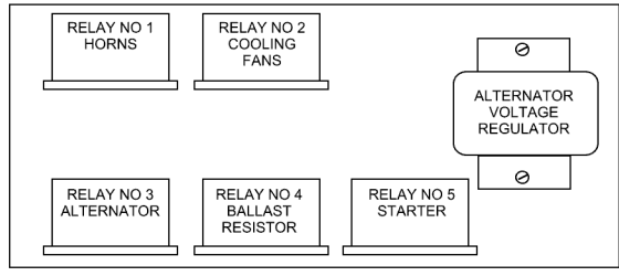
RELAY BOX LAYOUT
